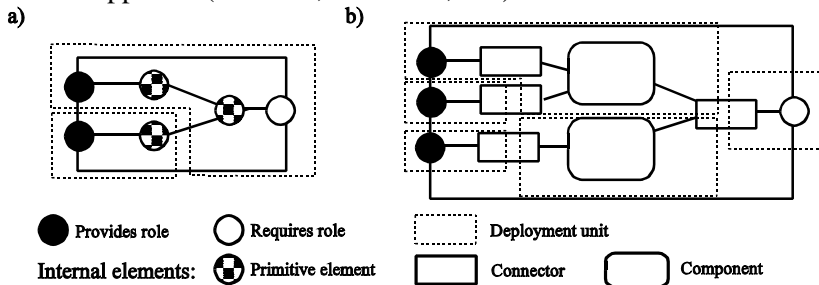
Figure 4. Connector model: a) simple architecture, b) compound architecture
