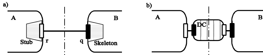
Figure 3. Deployment anomaly
