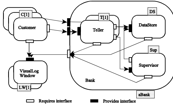
Figure 1. BankingDemo Architecture
