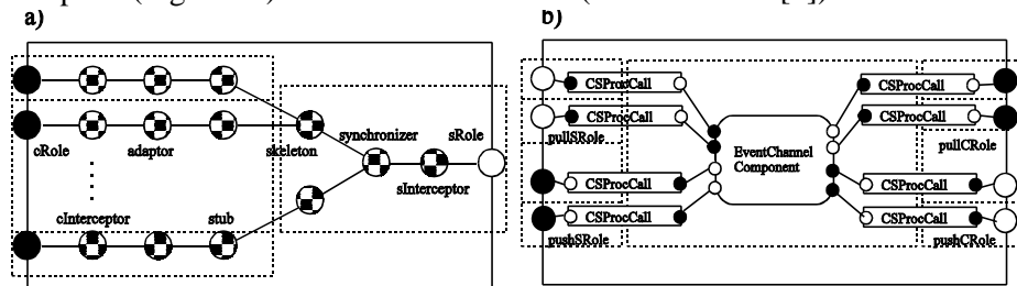
Figure 5. a) CSProcCall connector template, b) EventChannelDelivery connector template
