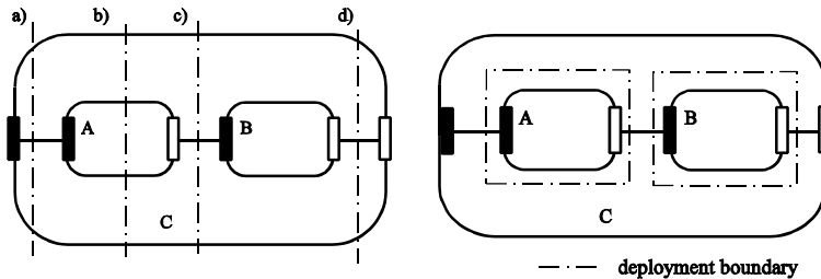
Figure 2. Deployment boundaries crossing interface ties
