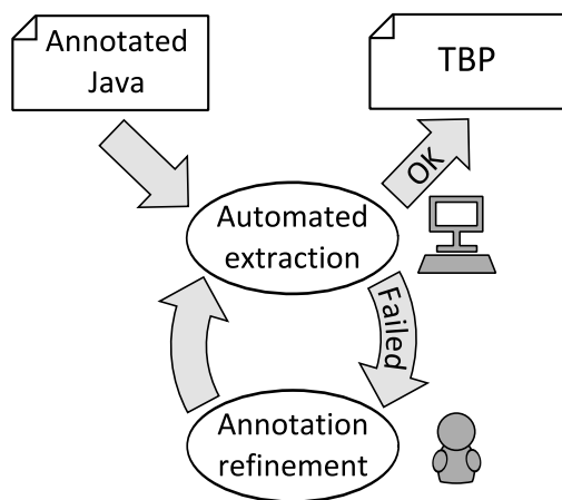
Figure 2. User assisted extraction of TBP specification
