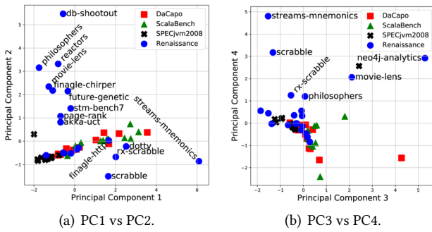
Figure 1. Scatter plots of benchmark scores over the first four principal components (PCs).
