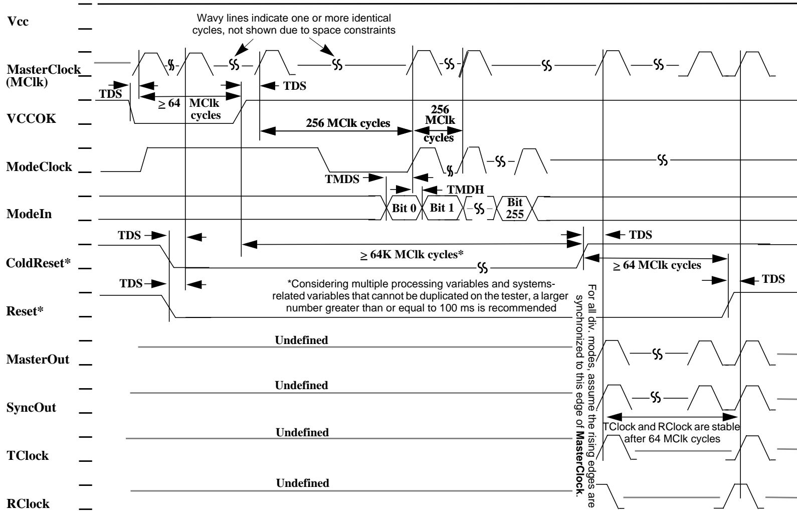
Figure 9-2 Cold Reset
