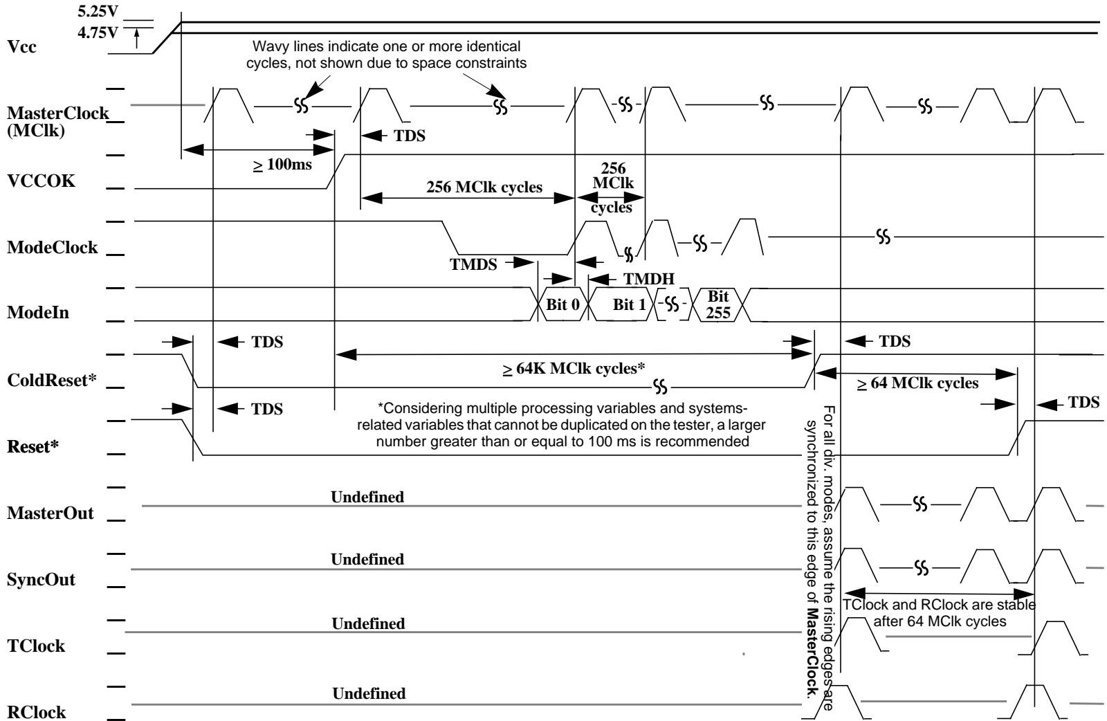
Figure 9-1 Power-on Reset
