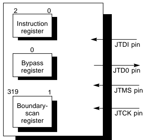
Figure 14-2 JTAG Interface Signals and Registers
