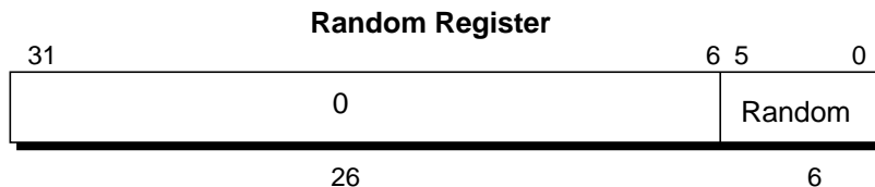
Figure 4-12 Random Register
