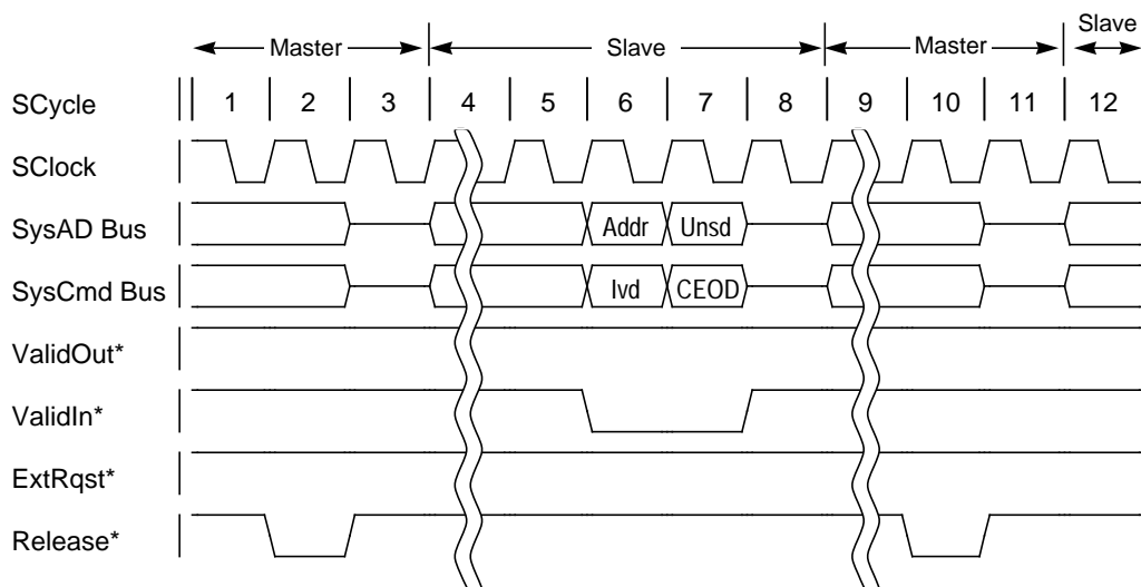
Figure 12-33 External Invalidate Request following an Uncompeled Change to Slave State
